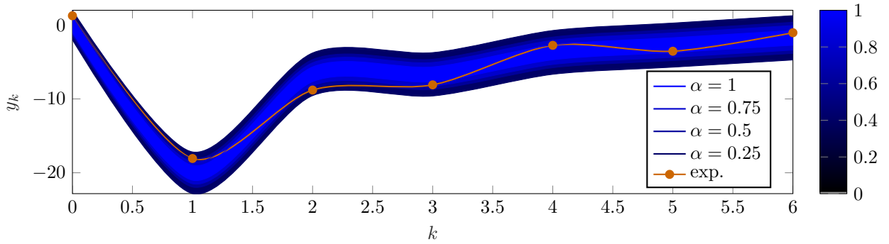
Figure 5. \alpha -cuts of the predicted measurement and simulated reference.
