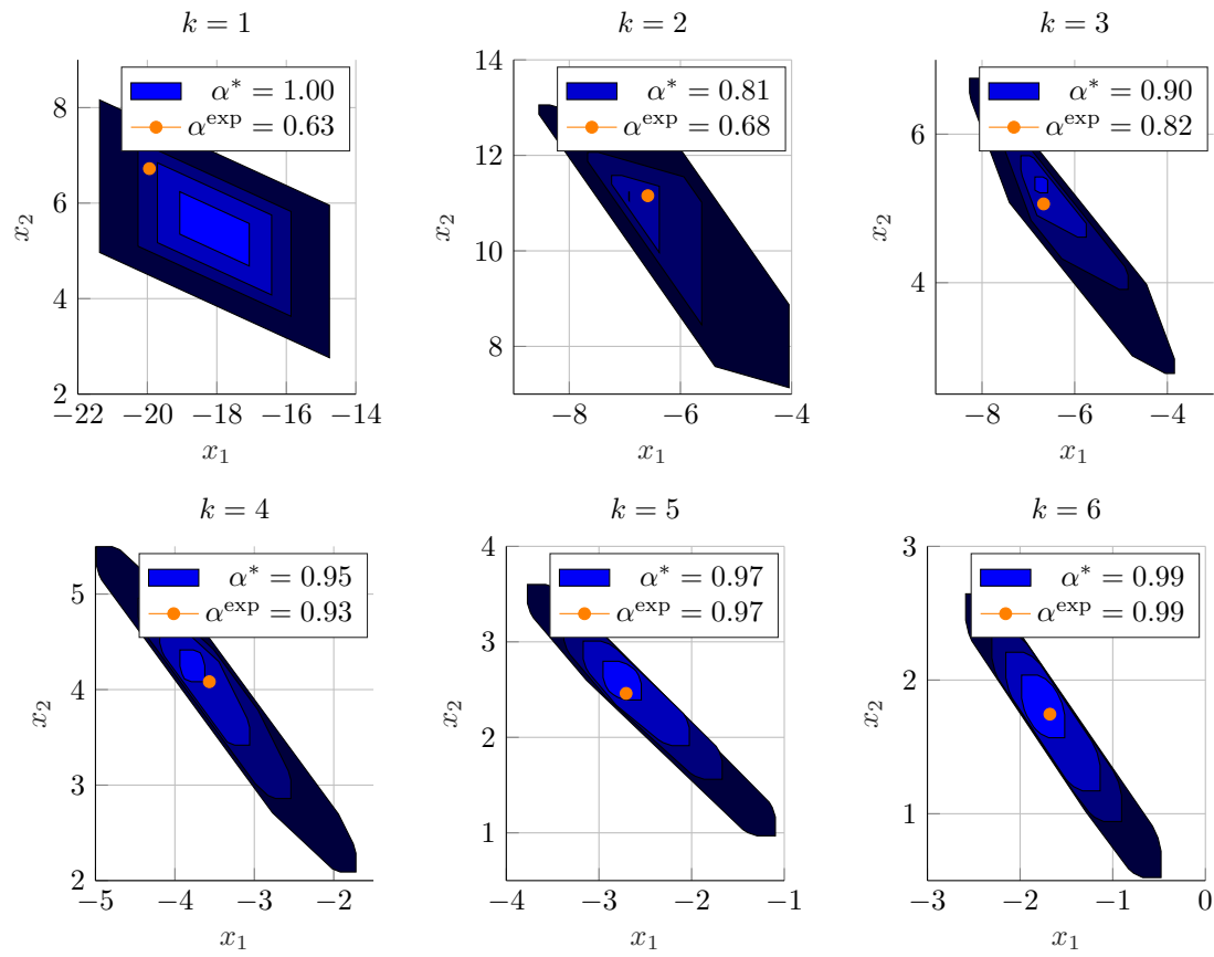
Figure 7. Confidence sets of the past system states (■) compared to the simulated reference (●). The coloring scheme represents the same \alpha -levels as in Fig. 1.
