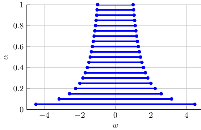
Figure 3. \alpha -cuts of the Chebychev possibility distribution of \widetilde{W} .
