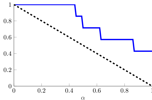
Figure 6. Empirical probabilities of the measurements y_k^{\text{exp}} being contained in the \alpha -cuts C_{Y_k}^\alpha compared to the guaranteed probability 1 - \alpha .
