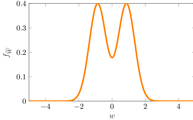
Figure 4. Probability density of \widetilde{W} in the reference simulation.
