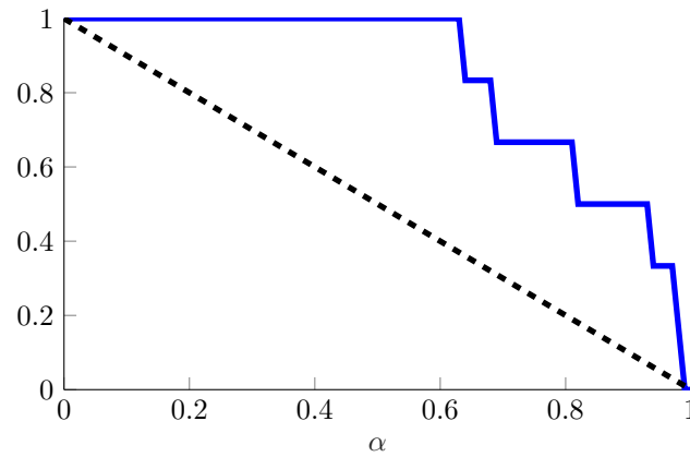
Figure 8. Relative frequency of the reference states \mathbf{x}_k being contained in the \alpha -cuts C_{\mathbf{x}_k}^\alpha compared to the guaranteed confidence level.
