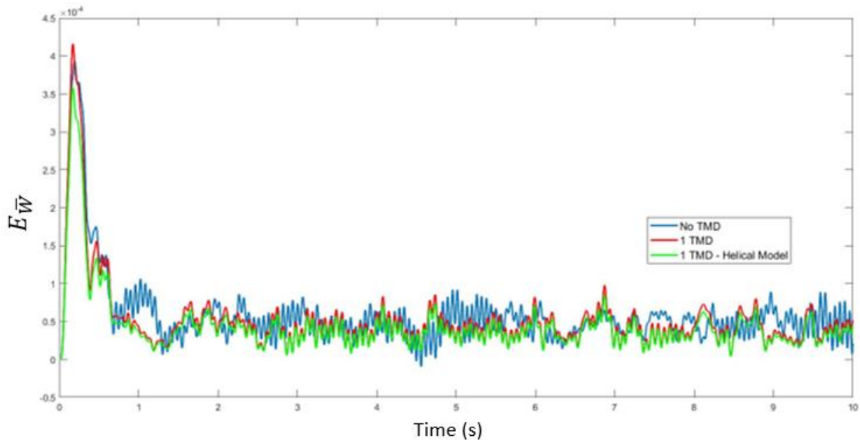
Figure 3. Mean Displacement.
